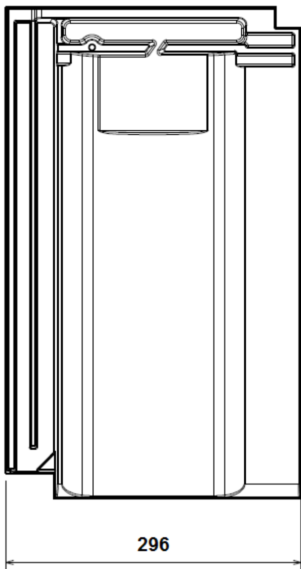
Figure 4 - Vue extradors
