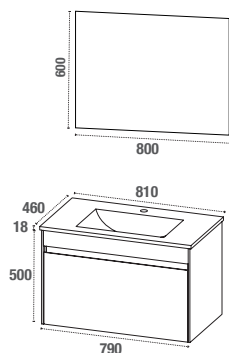
AGATE800CC AGATE800GP
