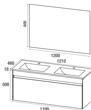
AGATE1200CC AGATE1200GP
