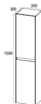
AGATE-C1500CC AGATE-C1500GP
